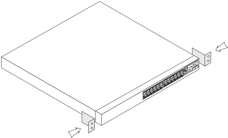
Figure 1-1. Bracket Installation for Rack Mounting
